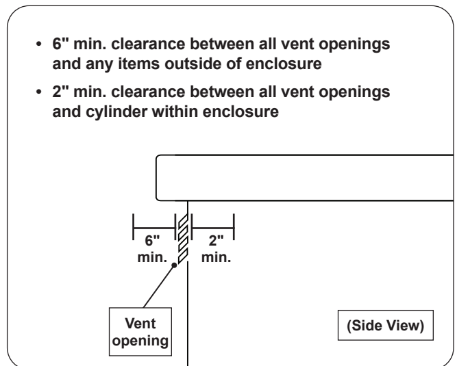
Fig. 17-1 Vent openings clearance
