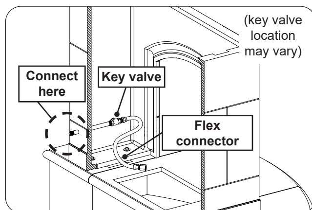
Fig. 25-2 Route gas supply (rear install)
