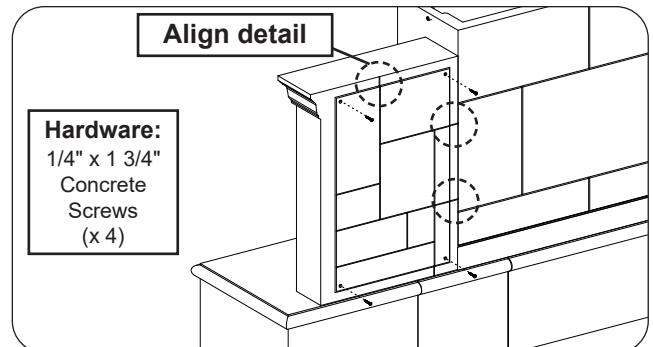
Fig. 26-2 Assemble rear side-wall (skip if n/a)
