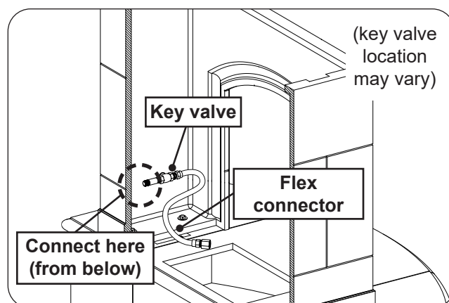
Fig. 25-3 Route gas supply (underneath install)
