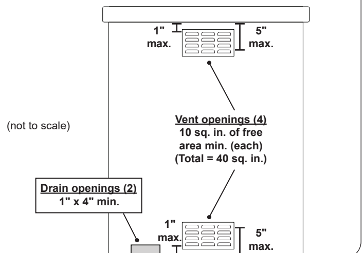
Fig. 17-2 Ventilation and drainage specifications (propane cylinder enclosure side view)
